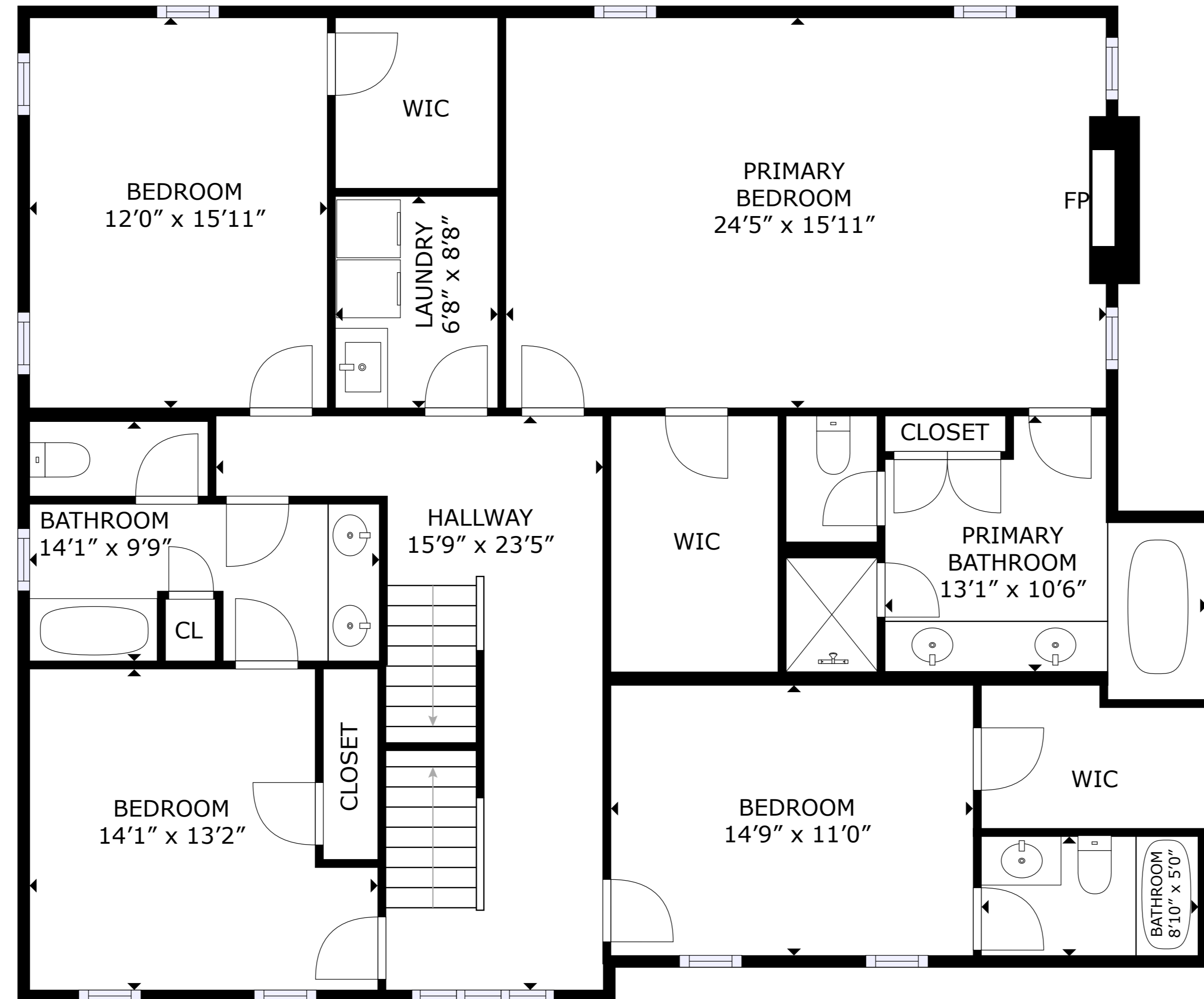
FLOOR 2
