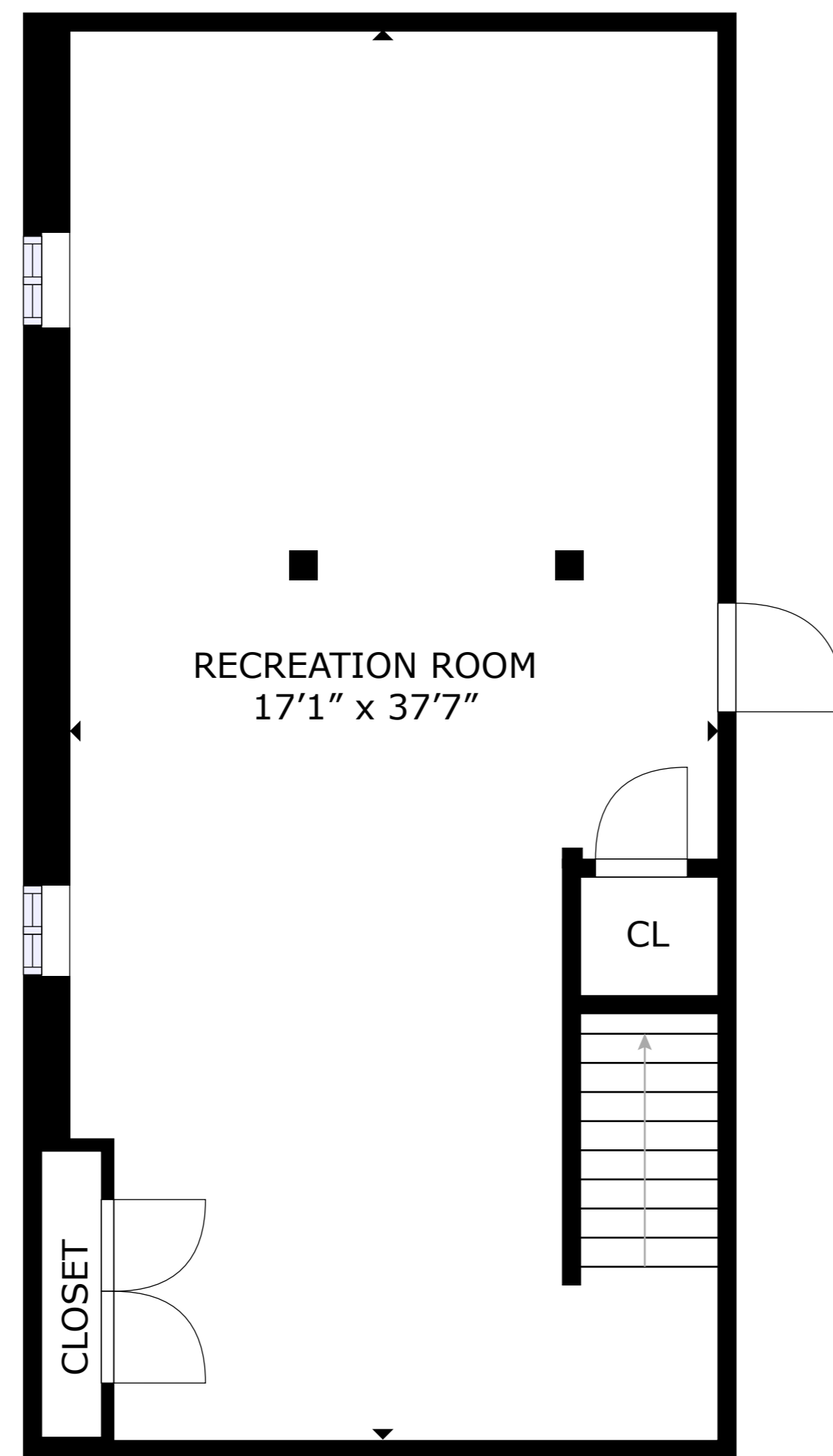
BASEMENT
